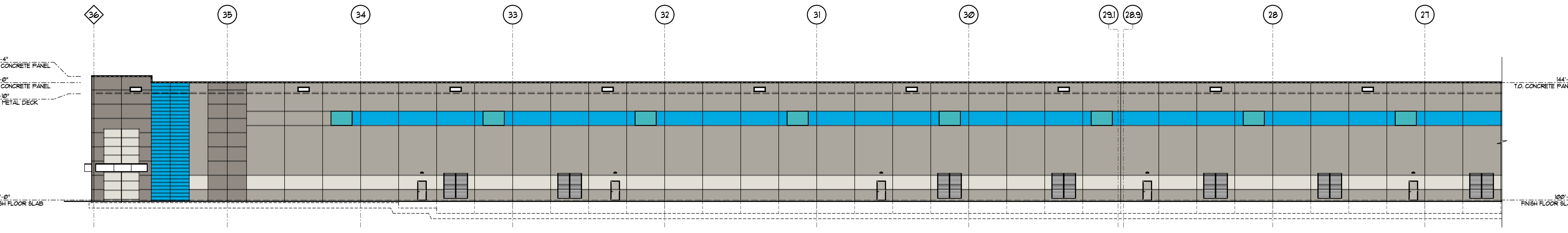
(E) PARTIAL EAST BUILDING ELEVATION SCALE 1/16" = 1'-0"
