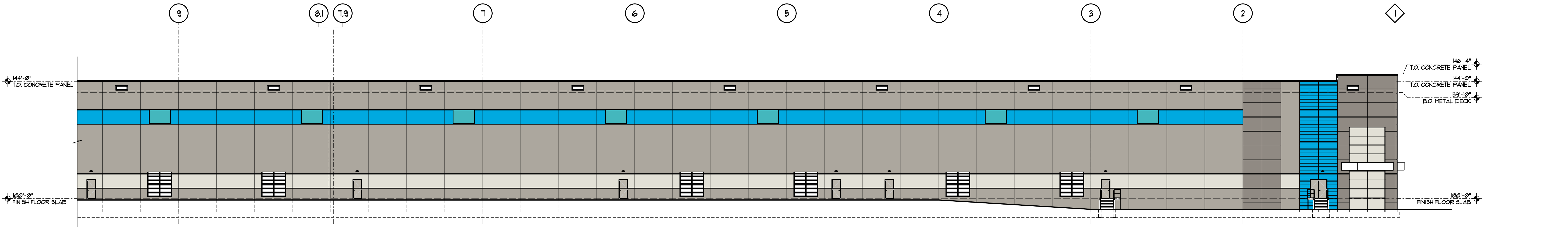
(B) PARTIAL EAST BUILDING ELEVATION SCALE 1/16" = 1'-0"
