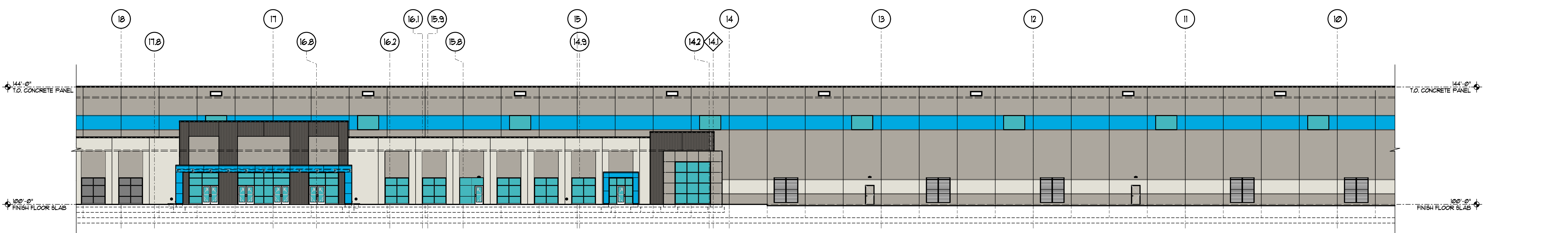
(C) PARTIAL EAST BUILDING ELEVATION SCALE 1/16" = 1'-0"
